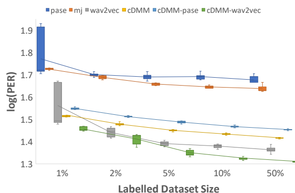
Figure 2: PER on WSJ eval92 dataset using features extracted from different models.
