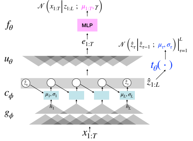
Figure 1: An illustration of the ConvDMM.
