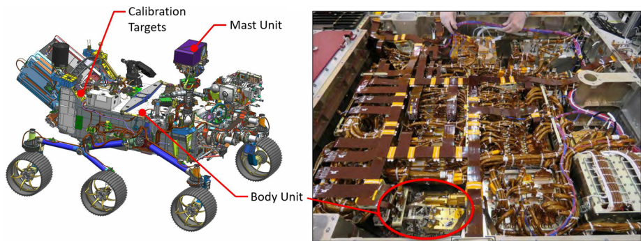
Fig. 3 Locations of the SuperCam units on the rover. The right side shows the rover body inverted, with the Body Unit circled. It is next to the RSM side of the rover to minimize the length of the fiber that transfers the optical signal from the mast unit. The rover's instrument and electronics bay is 1181 \times 1106 mm (length, left-right, x width)
