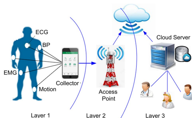
Fig. 1 WBAN architecture
