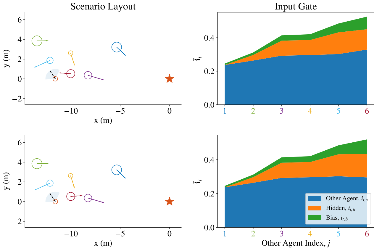
FIGURE 15. Gate Dynamics on Single Timestep. In the top row, one agent, near (-12,0), observes 6 neighboring agents. Other agent states are passed into the LSTM sequentially, starting with the furthest agent, near (-5, 3). The top right plot shows the impact of each LSTM cell input on the input gate as each agent is added to the LSTM: other agent state (bottom slice), previous hidden state (middle slice), and bias (top slice). The bottom row shows the same scenario, but the closest agent, near (-10,0), has a velocity vector away from the ego agent. Accordingly, the bottom right plot's bottom slice slightly declines from j = 5 to j = 6 , but the corresponding slice increases in the top right plot. This suggests the LSTM has learned to put more emphasis on agents heading toward the ego agent, as they are more relevant for collision avoidance.
