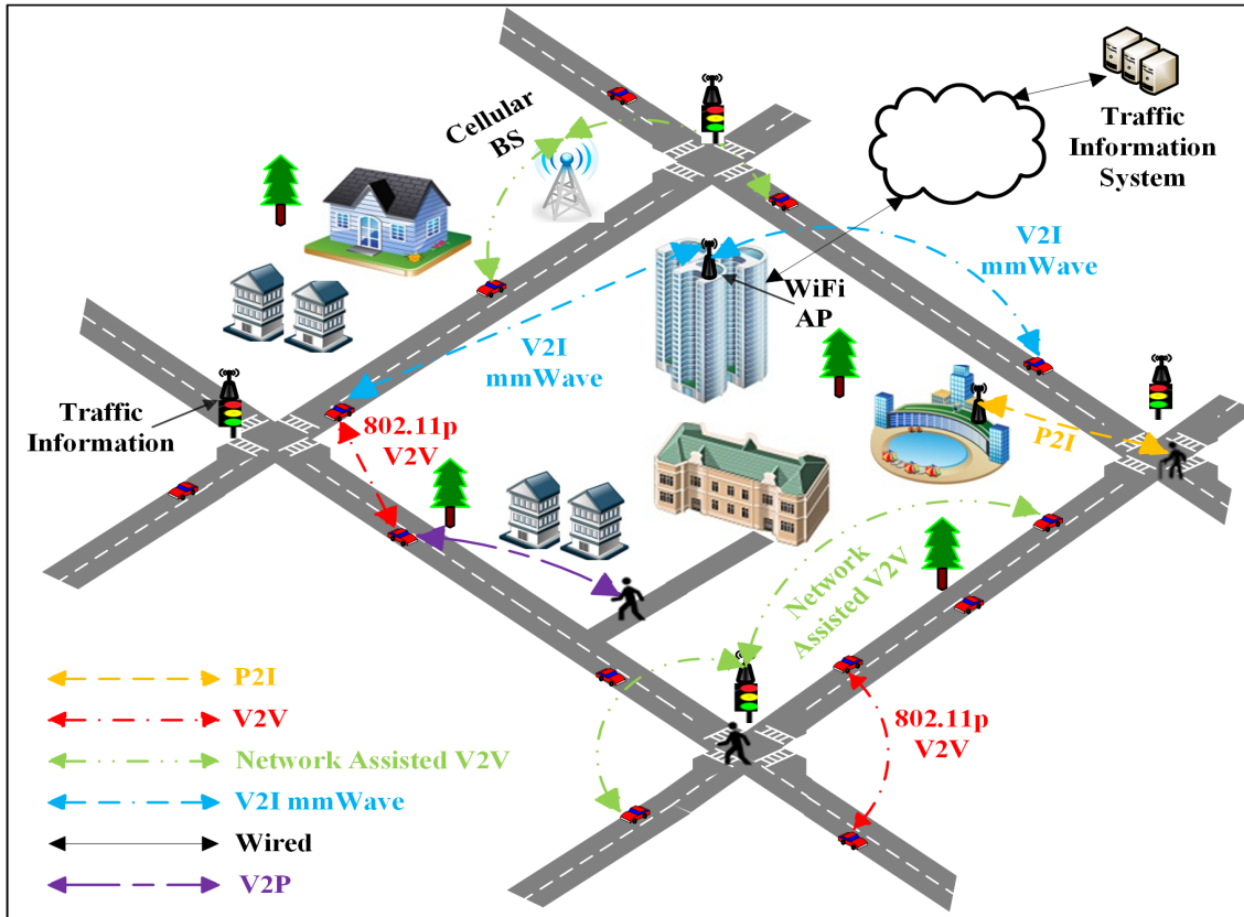
FIGURE 2. V2X communication infrastructure using different technologies.
