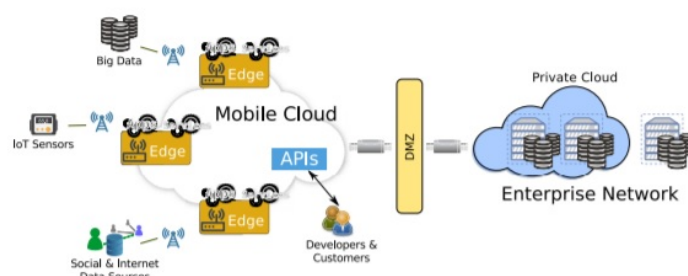
FIGURE 4. Mobile Edge Computing Architecture
