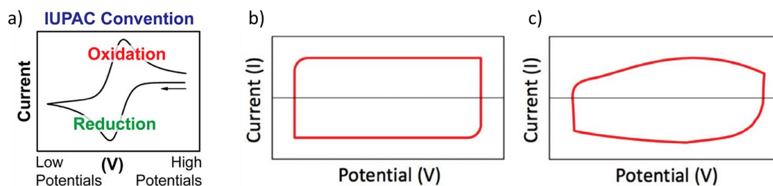
Figure 2.6 IUPAC convention for the CV (a) and examples of CV curves for an electrical double layer capacitor (b) and pseudocapacitor (c). Adapted from [21] (a) and [22] (b, c).
