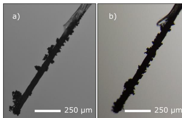
Figure 4.3 Overgrown PEDOT clusters in standard PEDOT:C10 4 coating a) and thinner layer b).
