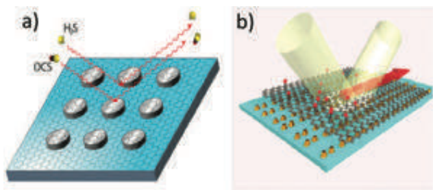
Fig. 119 (a) Illustration of graphene-passivated Ag nanoantennas fabricated in a square array. The graphene layer prevents the reaction of trace atmospheric hydrogen sulfide ( \text{H}_2\text{S} ) and carbonyl sulfide (OCS) with the Ag surface. Adapted from ref. 2327. (b) Scheme of a square array of Au double-dots on a glass substrate covered by hydrogenated graphene. Adapted from ref. 2310.
