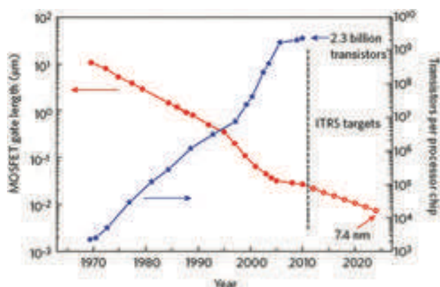
Fig. 57 Evolution of MOSFET gate length integrated circuits (filled red circles). The ITRS targets a gate length of 7.4 nm in 2025 (open red circles). With the decrease of gate lengths, the number of transistors per processor increased (blue stars). New materials, like graphene, are needed to maintain these trends. 433
