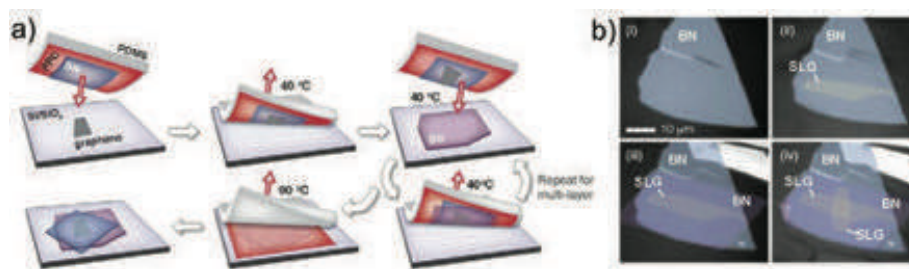
Fig. 50 Layer by layer assembly process. (a) Schematic diagram showing the steps to make a BN-SLG-BN stack or a multiple-layer stack with device layer (graphene) never exposed to any polymer or solvent. (b) Optical images showing in sequence a BN flake on poly-propylene carbonate (PPC) and film picking. Adapted from ref. 999.
