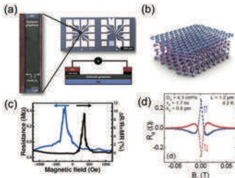
Fig. 71 (a) Typical two-terminal local spin valve device. The width of graphene channel on SiC is 10 \mu\text{m} , and the distance between the two \text{Al}_2\text{O}_3/\text{Co} electrodes is L = 2 \mu\text{m} . The optical image shows the entire structure, including contact pads. (b) Atomic arrangement of SLG on SiC. (c) Large local resistance spin signals measured at 4 K. (d) Oscillating and decaying device non-local resistance as a function of the applied magnetic field (Hanle measurement). Adapted from ref. 223, 1300.
