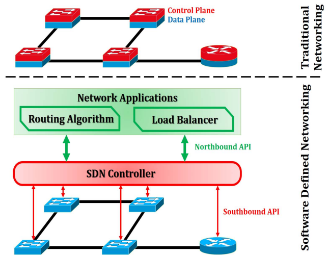
Fig. 2. SDN versus traditional networking architectures.
