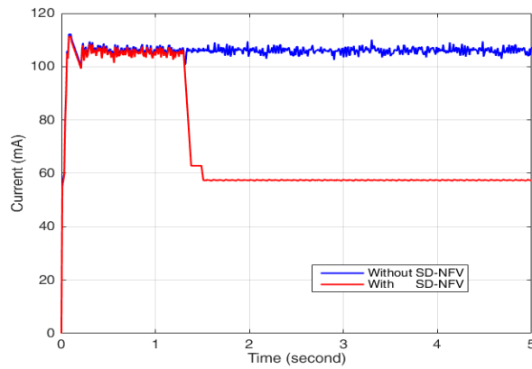
Fig. 12. First 6 s of the network initialization phase.
