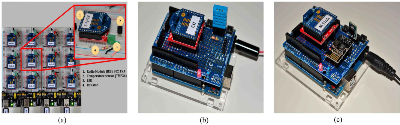
Fig. 4. M2M sensor node prototypes used in the cloud-based 6LoWPAN testbed. (a) Simple node. (b) Advanced node. (c) Sink node.
