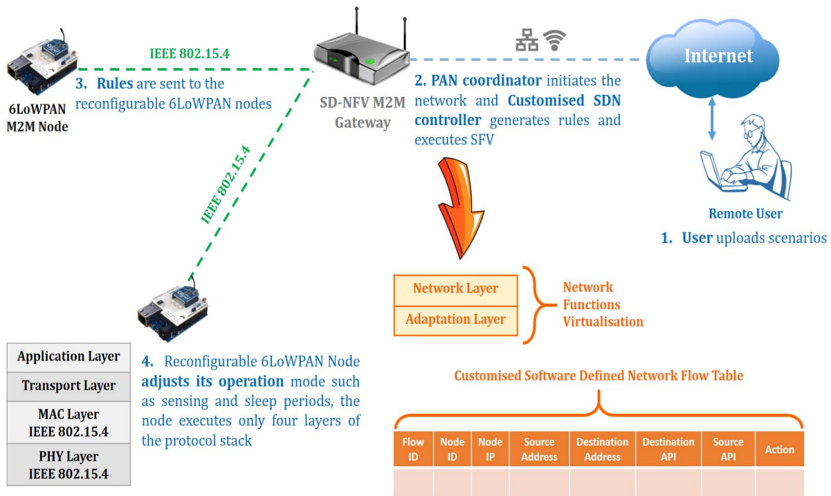
Fig. 7. Proposed architecture of the SD-NFV gateway using cloud-based 6LoWPAN testbed.
