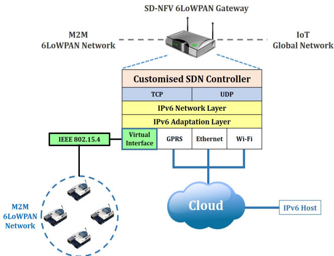
Fig. 8. 6LoWPAN cloud connectivity through SD-NFV gateway.
