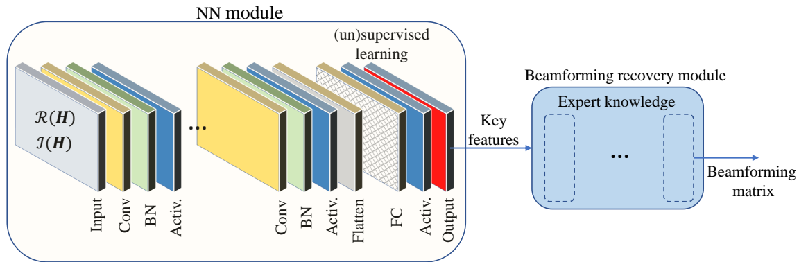
FIGURE 8. Feature-based DLB framework [147] with two main modules: NN and beamforming recovery. The NN module consists of input, convolutional (conv), batch normalization (BN), activation (activ.), flatten, fully connected (FC), and output layers. The NN module outputs the key features, which allow the beamforming matrix to be constructed by leveraging the expert knowledge in the beamforming recovery module.
