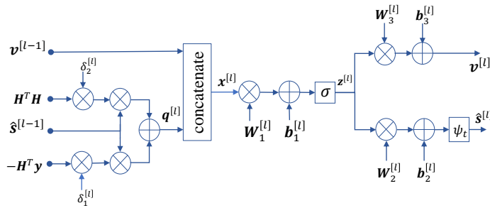
FIGURE 7. Illustration of layer l of the DetNet [11], [49], [118].
