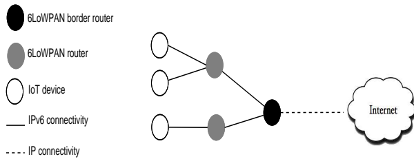
FIGURE 8. 6LoWPAN architecture
