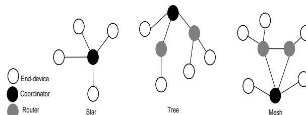
FIGURE 6. ZigBee topologies
