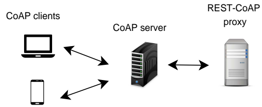
FIGURE 10. CoAP architecture
