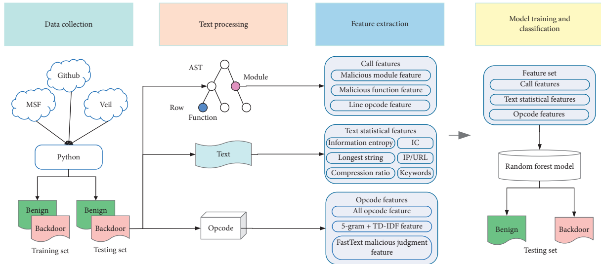
FIGURE 1: Architecture of PBDD.
