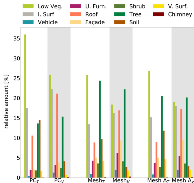
Fig. 7. Class distributions of the training set T and the validation set V both for H3D(PC) and H3D(Mesh). For the mesh, the relative class distribution is given in terms of i) the face count and ii) the area A of faces. Unlabeled faces are not considered in this figure.
