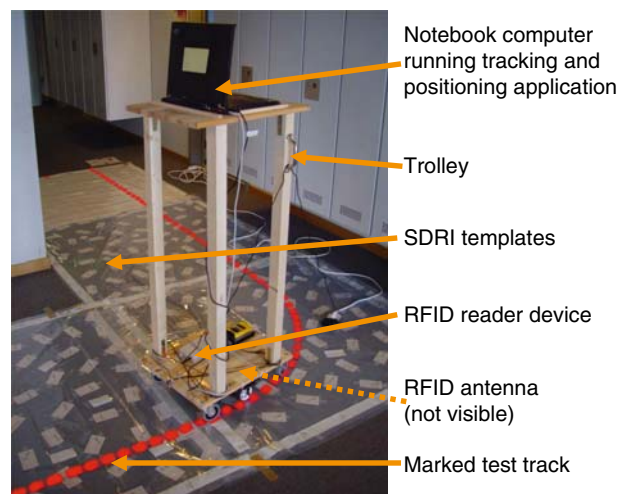
Fig. 2 Measurement trolley and prepared test track
