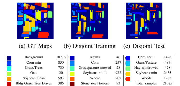
Fig. 15: The type associated with the land-cover classes and number of available samples in the Indian Pines (IP) dataset. Moreover, Spatially disjoint training and test samples for the IP dataset are also presented.
