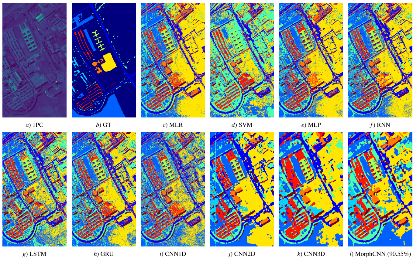
Fig. 20: Classification Maps obtained by MLR [321], SVM [322], MLP [69], RNN [70], LSTM [323], GRU [324], CNN-1D [218], CNN-2D [325], CNN-3D [326] and MorphCNN [196] on the disjoint train-test dataset for the UP scene.
