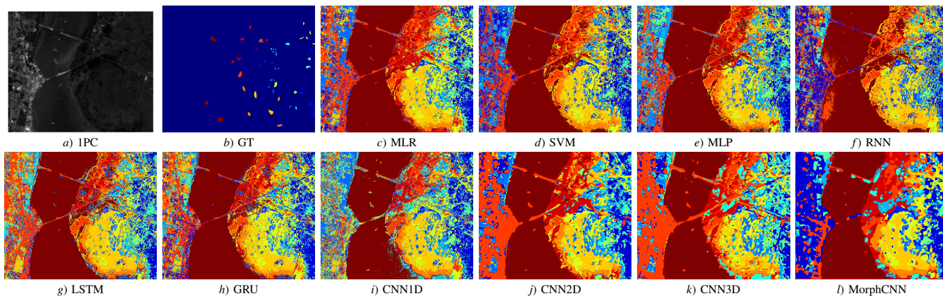
Fig. 23: Classification Maps obtained by MLR [321], SVM [322], MLP [69], RNN [70], LSTM [323], GRU [324], CNN-1D [218], CNN-2D [325], CNN-3D [326] and MorphCNN [196] on the disjoint train-test dataset for the KSC scene.
