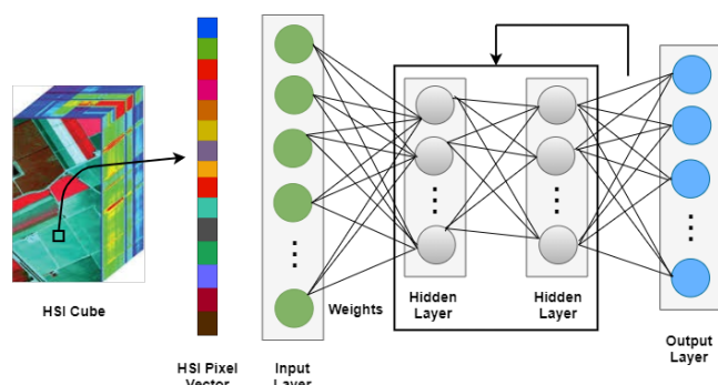
Fig. 11: RNN architecture
