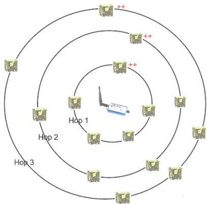
FIGURE 5. A network with 30 nodes and 3-hops
