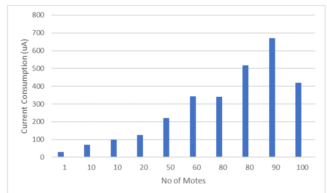
FIGURE 3. Variation of current consumption with No. of Motes
