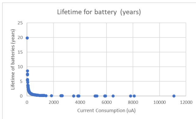
FIGURE 17. Battery lifetime Vs. current consumption
