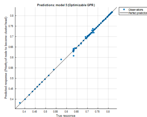
FIGURE 15. Predicted Vs true response for CH selection
