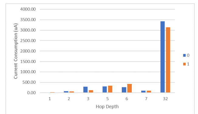
FIGURE 4. Variation of current consumption for different hop depths (0 – Routing, 1- Non-routing)
