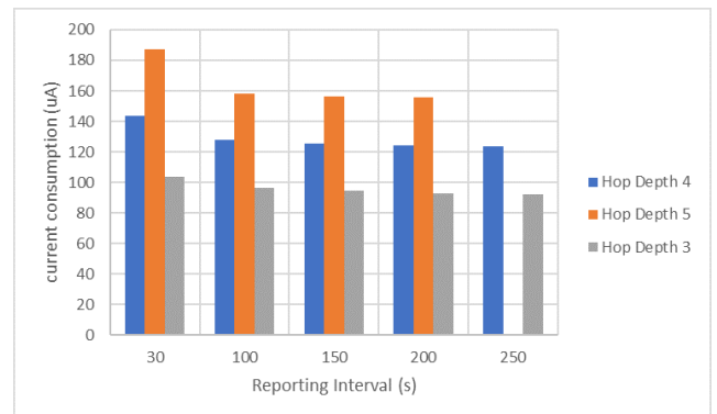
FIGURE 2. Variation of current consumption with reporting interval at different hop depth
