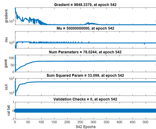
FIGURE 14. Optimized values of different hyperparameters
