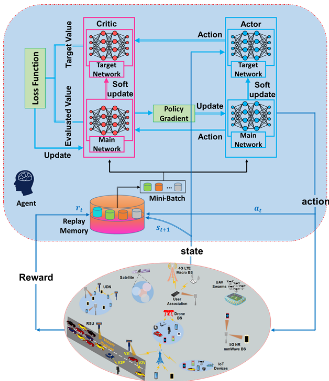
Fig. 10. Illustration of the DDPG actor-critic architecture [88].
