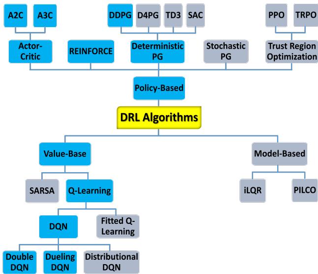
Fig. 7. Taxonomy of all DRL algorithms [37]. Algorithms colored in blue are covered in Section III.
