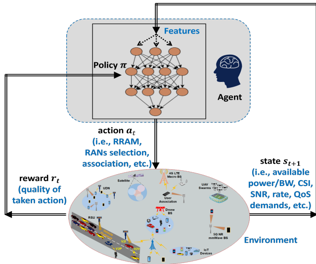
Fig. 8. Framework of DRL models [15].
