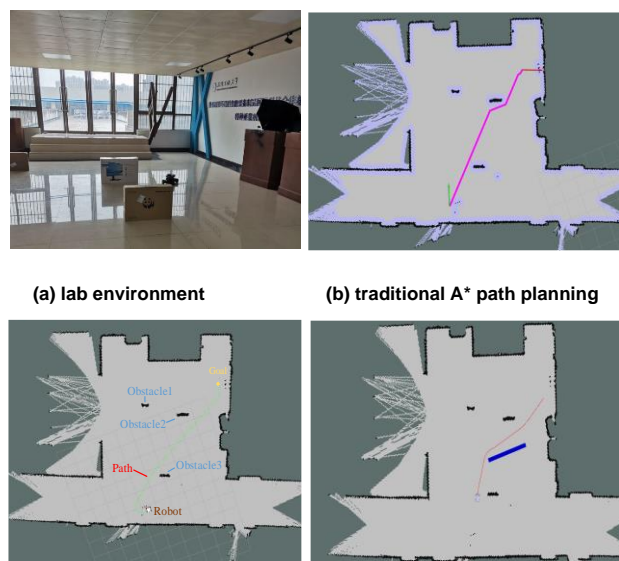
(a) lab environment (b) traditional A* path planning (c) fusion algorithm path planning (d) path planning under dynamic obstacles.
