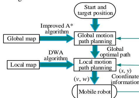
FIGURE 13. Hybrid algorithm planning diagram.
