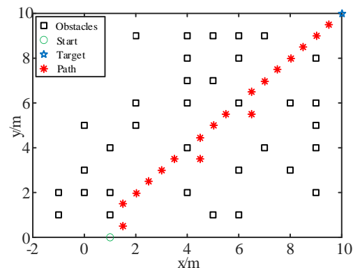
FIGURE 5. Path planning results of the traditional A* algorithm.
