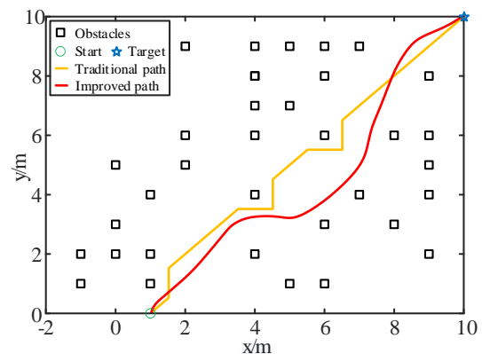
FIGURE 15. Path simulation diagram of hybrid algorithm.
