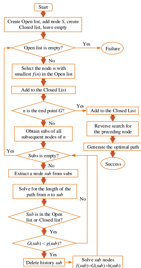
FIGURE 3. A* algorithm flowchart.
