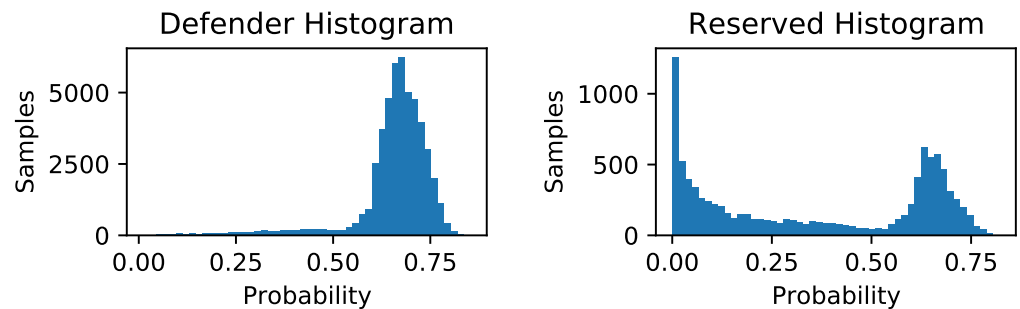
Figure A1. Histogram of predicted probabilities.
