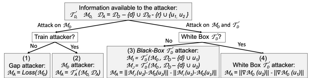
Figure 2. Taxonomy of LTU Attacker. Top: Any LTU Attacker has available the Defender trainer \mathcal{T}_D , the trained Defender model \mathcal{M}_D , and attack data \mathcal{D}_A including (almost) all the Defender data \mathcal{D}_D and Reserved data \mathcal{D}_R \mathcal{D}_A = \mathcal{D}_D - \{\text{membership}(d)\} \cup \mathcal{D}_R - \{\text{membership}(r)\} . However, it may use only part of this available knowledge to conduct attacks. r and d are two labeled examples belonging \mathcal{D}_R and \mathcal{D}_D , respectively, and u_1 and u_2 are two unlabeled examples, one from \mathcal{D}_R and one from \mathcal{D}_D (ordered randomly). Bottom Left: Attacker \mathcal{M}_A targets only the trained Defender model \mathcal{M}_D . Bottom Right: \mathcal{M}_A targets both \mathcal{M}_D and its trainer \mathcal{T}_D .
