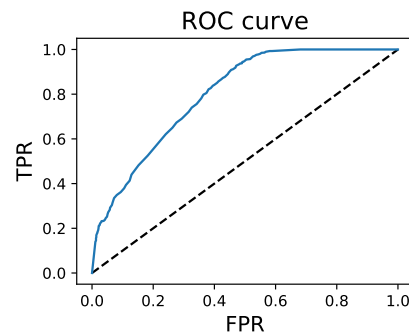
Figure 4. The ROC curve for the membership predictions from a model trained on Location-30 and defended by MemGuard. The AUROC was 0.8, and the TPR was much higher than the FPR in the low FPR regime.
