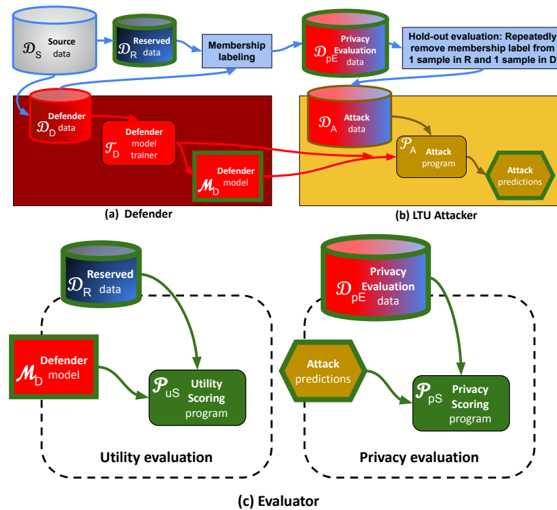
Figure 1. Methodology flow chart. (a) Defender: Source data are divided into Defender data , to train the model under attack ( Defender model ) and Reserved data to evaluate such a model. The Defender model trainer creates a model optimizing a utility objective, while being as resilient as possible to attacks. (b) LTU Attacker: The evaluation apparatus includes an LTU Attacker and an Evaluator : The evaluation apparatus performs a hold-out evaluation leaving two unlabeled examples (LTU) by repeatedly providing the LTU Attacker with ALL of the Defender and Reserved data samples, together with their membership origin , hiding only the membership label of 2 samples. The LTU Attacker must turn in the membership label (Defender data or Reserved data) of these 2 samples (Attack predictions). (c) Evaluator: The Evaluator computes two scores: LTU Attacker prediction error ( Privacy metric ), and Defender model classification performance ( Utility metric ).
