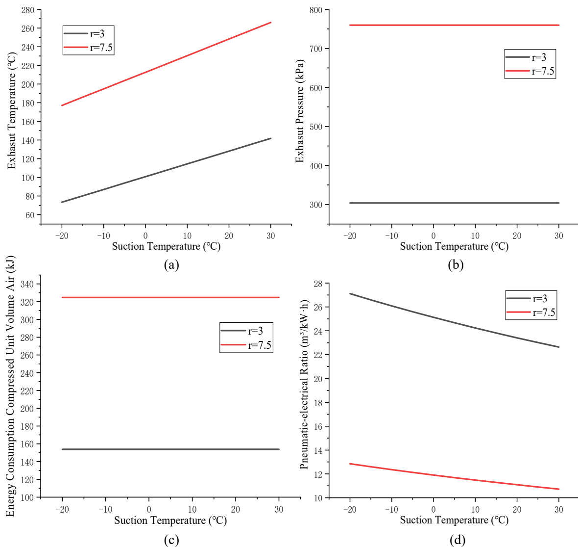
Figure 8. Changes in air compressor system parameters when suction temperature T_{in} changes: (a) Exhaust temperature; (b) Exhaust pressure; (c) Energy consumption compressed unit volume air; (d) Pneumatic-electrical ratio.
