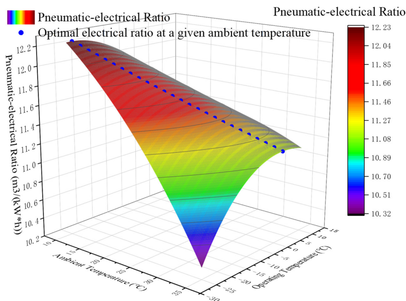
Figure 14. The relationship between the pneumatic-electricity ratio and operating temperature of the system under different ambient temperatures T_{en} .
