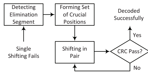
Figure 8. The procedure of double-shifting when the single shift at T positions fails.
