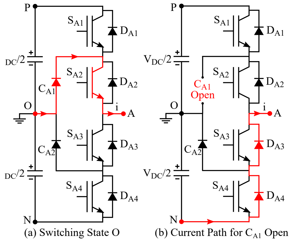
Figure 8. C_{A1} OC switch fault.
