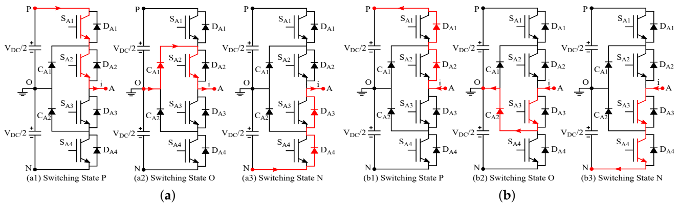
Figure 3. Switching state circuits based on current direction for pole A. (a) Switching states P, O, N for i > 0 . (b) Switching states P, O, N for i < 0 .
