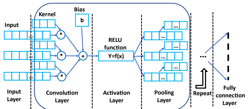
Figure 15. Structure of 1-D CNN network.
