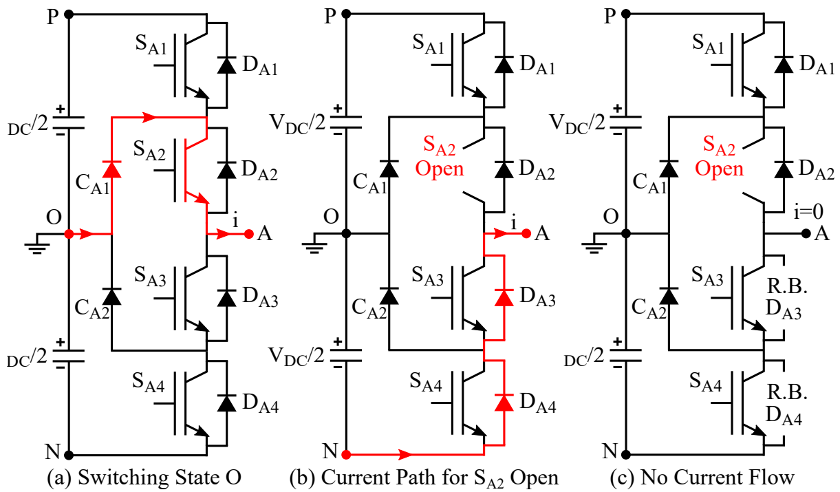
Figure 5. Circuit diagram for S_{A2} open switch fault.
