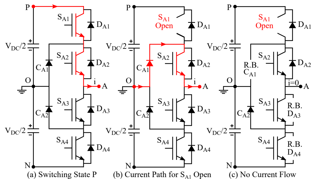
Figure 4. Circuit diagram for S_{A1} open switch fault.
