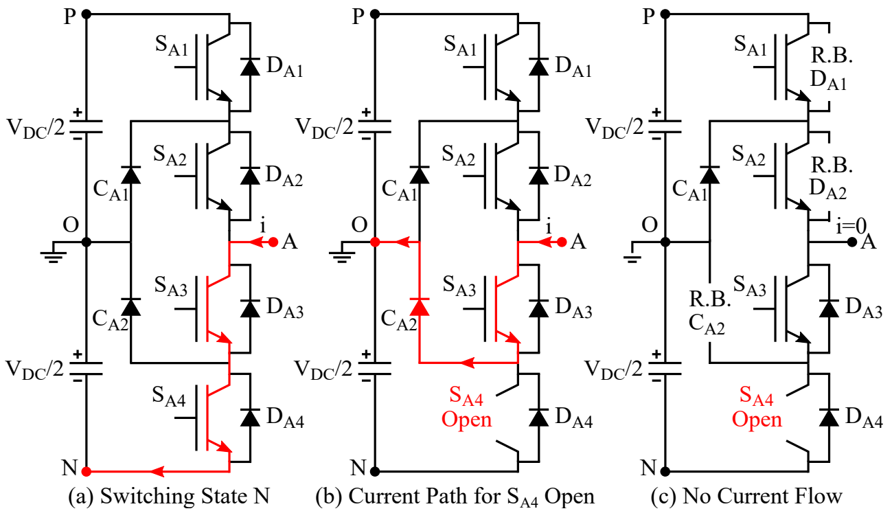
Figure 7. Circuit diagram for S_{A4} open switch fault.
