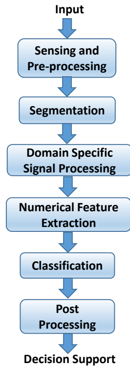
Figure 12. Block diagram representation of signal processing-based fault diagnostic method.
