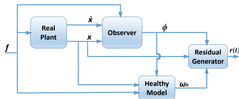
Figure 13. Block diagram representation of model-based fault diagnosis method.
