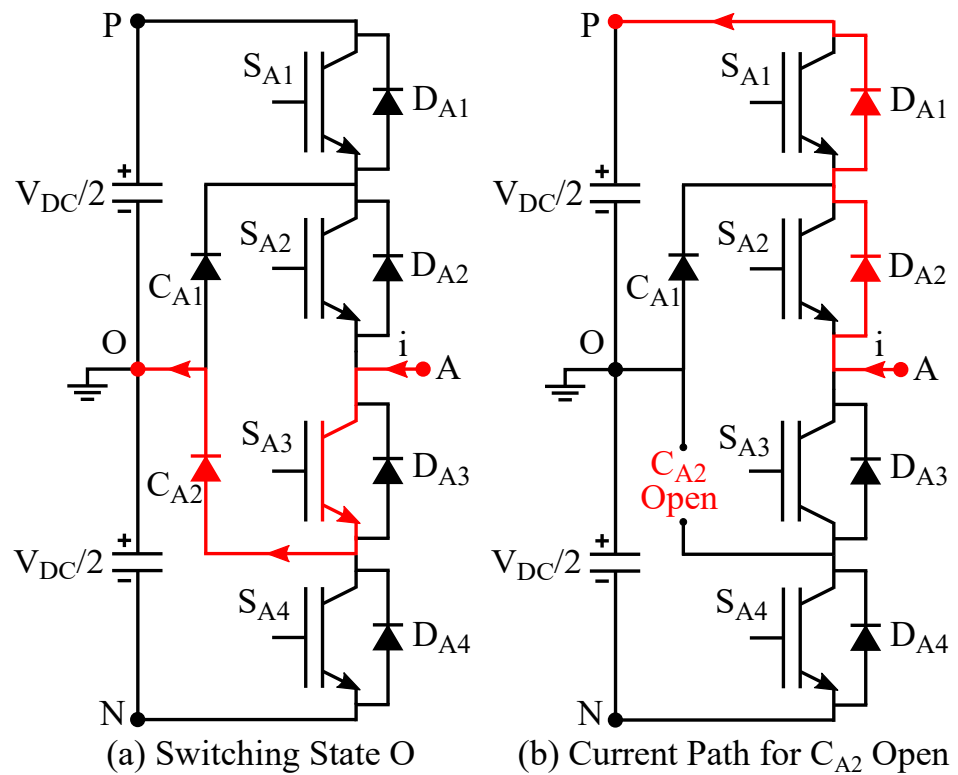
Figure 9. C_{A2} OC switch fault.
