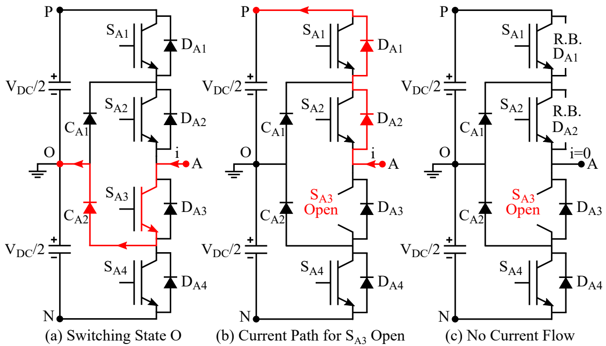
Figure 6. Circuit diagram for S_{A3} open switch fault.
