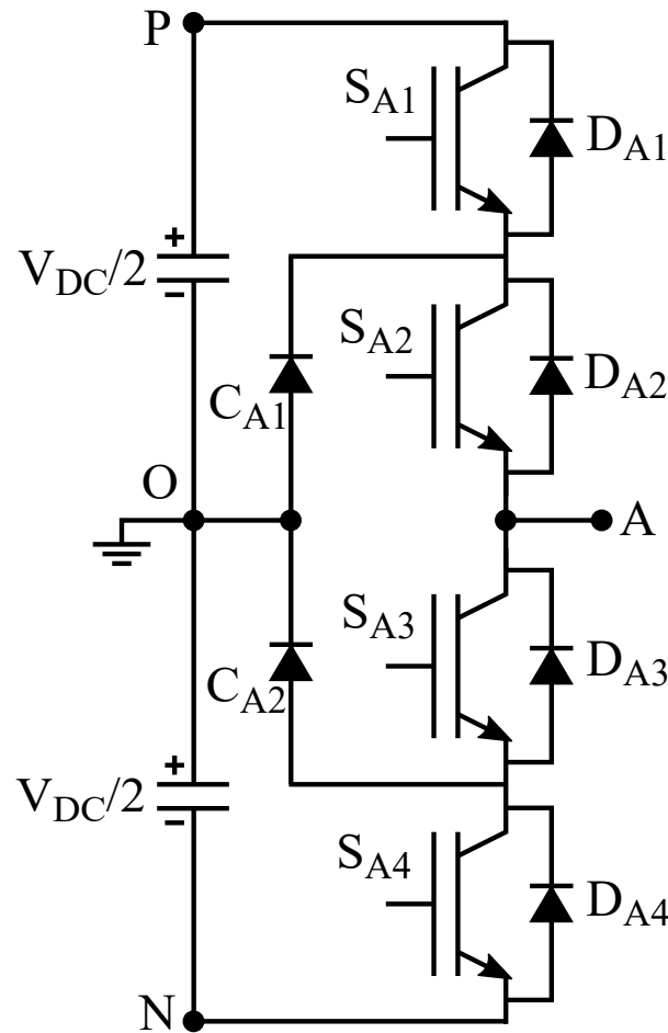
Figure 2. A leg of the NPC inverter.
