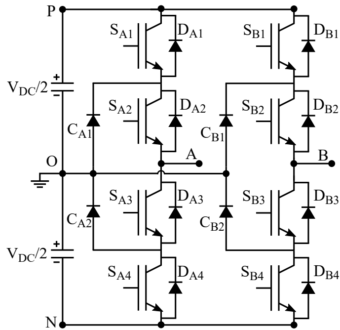
Figure 1. Single-phase neutral point clamped inverter.
