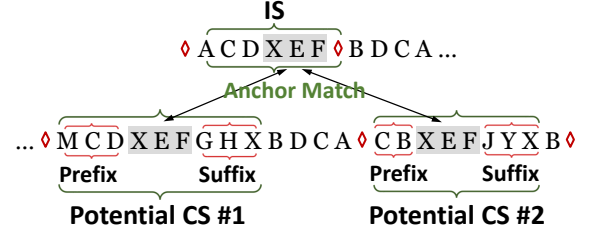
Figure 6. An overview of missing data recovery: the anchor instructions are “XEF”.
