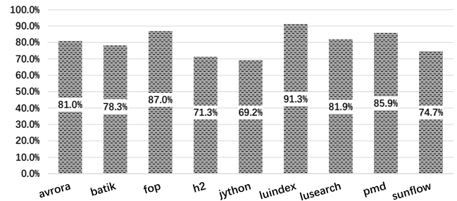
Figure 7. JPortal’s overall accuracy, using profiles collected by the instrumentation-based approach as ground truth.
