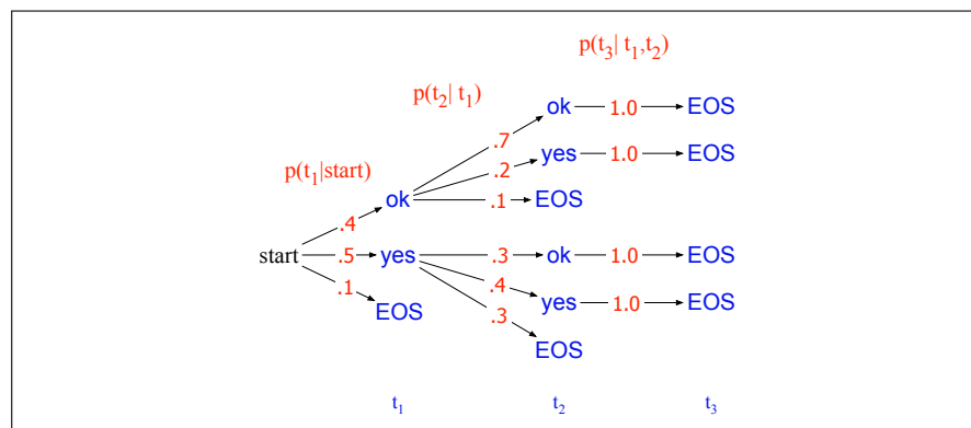
Figure 13.7 A search tree for generating the target string T = t_1, t_2, \dots from vocabulary V = \{\text{yes, ok, } \langle s \rangle\} , showing the probability of generating each token from that state. Greedy search chooses yes followed by yes , instead of the globally most probable sequence ok ok .
