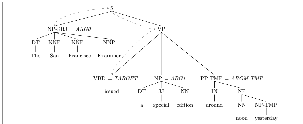
Figure 21.5 Parse tree for a PropBank sentence, showing the PropBank argument labels. The dotted line shows the path feature NP\uparrow S\downarrow VP\downarrow VBD for ARG0, the NP-SBJ constituent The San Francisco Examiner .
