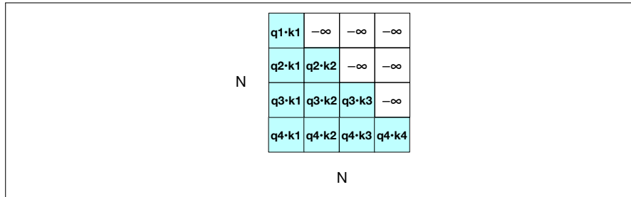
Figure 9.9 The N \times N \mathbf{Q}\mathbf{K}^T matrix showing the q_i \cdot k_j values, with the upper-triangular portion of the comparisons matrix zeroed out (set to -\infty , which the softmax will turn to zero).
