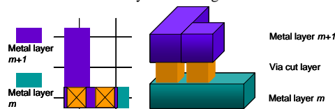
Fig. 1 Illustration for redundant via insertion.
