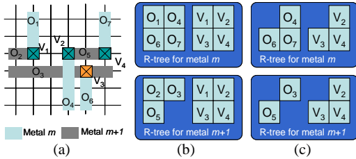
Fig. 6. Illustration for IGCA .
