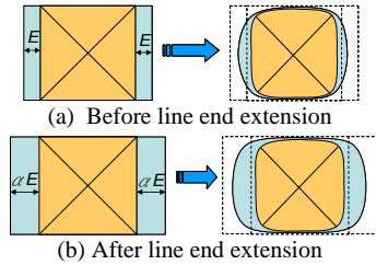
Fig. 2. Via pattern distortions.
