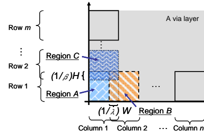
Fig. 10. Illustration for the via regions.
