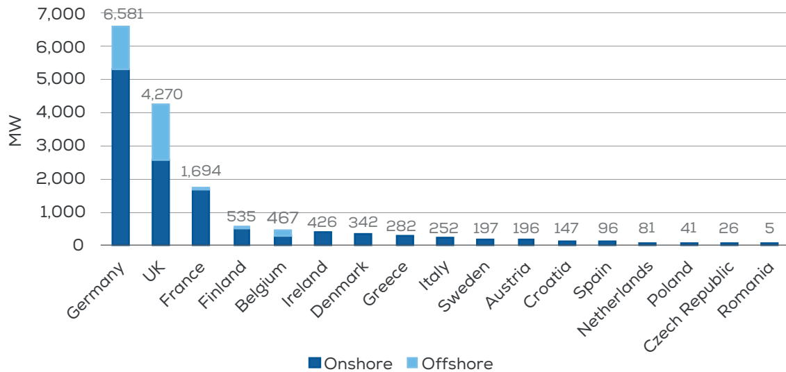
FIGURE 11 2017 installed wind energy capacity onshore and offshore. Total: 15,638 MW
