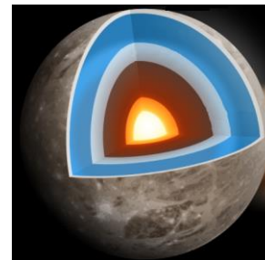
Figure 195: Ganymede's Interior
