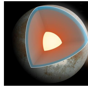
Figure 194: Europa's Interior
