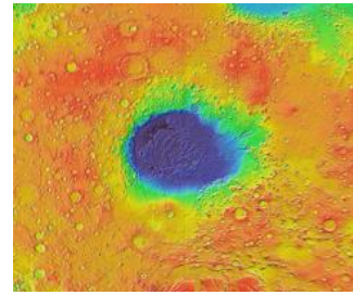
Figure 160: Hellas Basin
