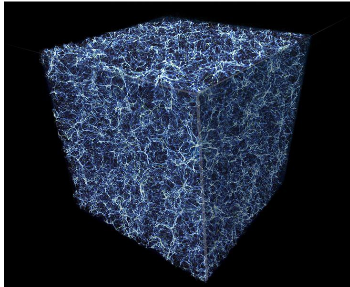
Figure 9: The Universe
