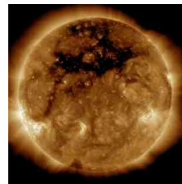
Figure 293: Coronal Hole
