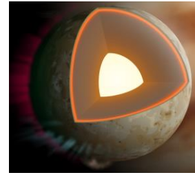
Figure 193: Io's Interior
