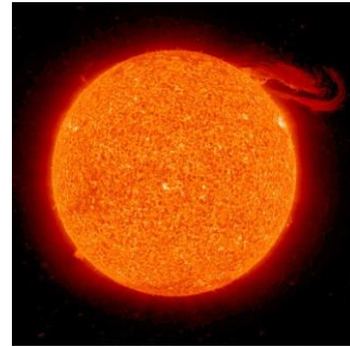
Figure 291: Solar Prominence
