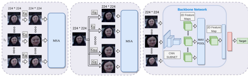
Figure 2: MSA (right) and data pre-processing for static (middle) and sequence (left) model.
