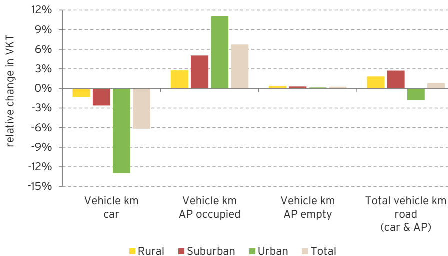
Figure 4.3.4. Change in vehicle-kilometres travelled (VKT) per day resulting from the introduction of an AP system in Germany by type of area (relative to total VKT without the AP system) compared to scenario „Technology breakthrough“
