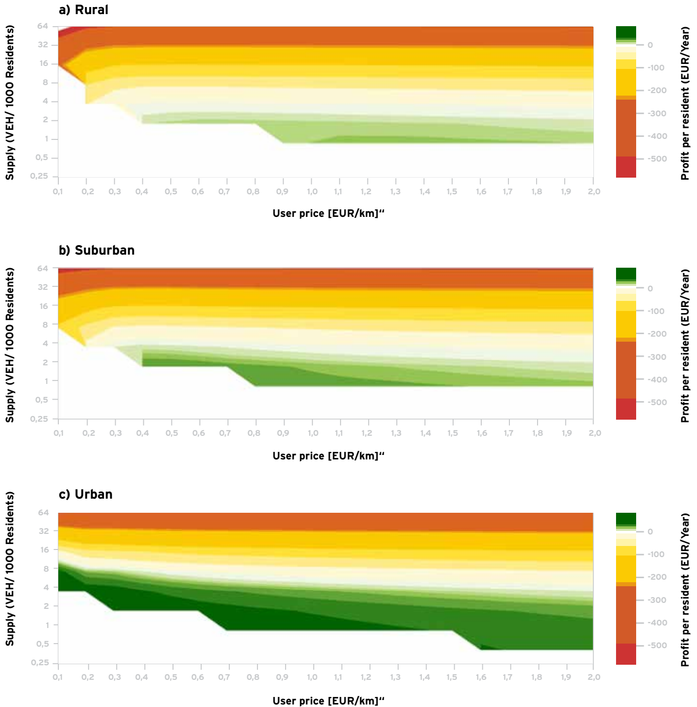
Figure A.3.3: AP-Operator profit per inhabitant and year as a function of user price (€/km) and level of provision (AP vehicles/1,000 residents) for different types of areas in Germany
