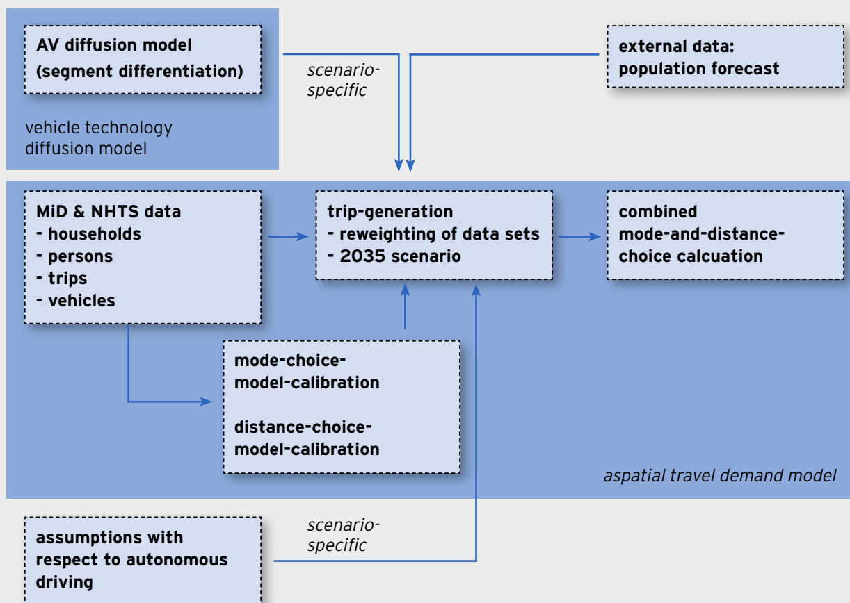
Figure A.3.1: Model scheme of the combined model approach for AV application
