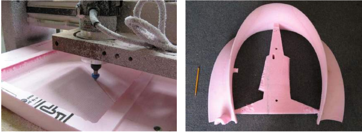
Fig. 11: (a) The milling machine used to make master patterns; (b) the smaller master segment obtained by CNC milling.
