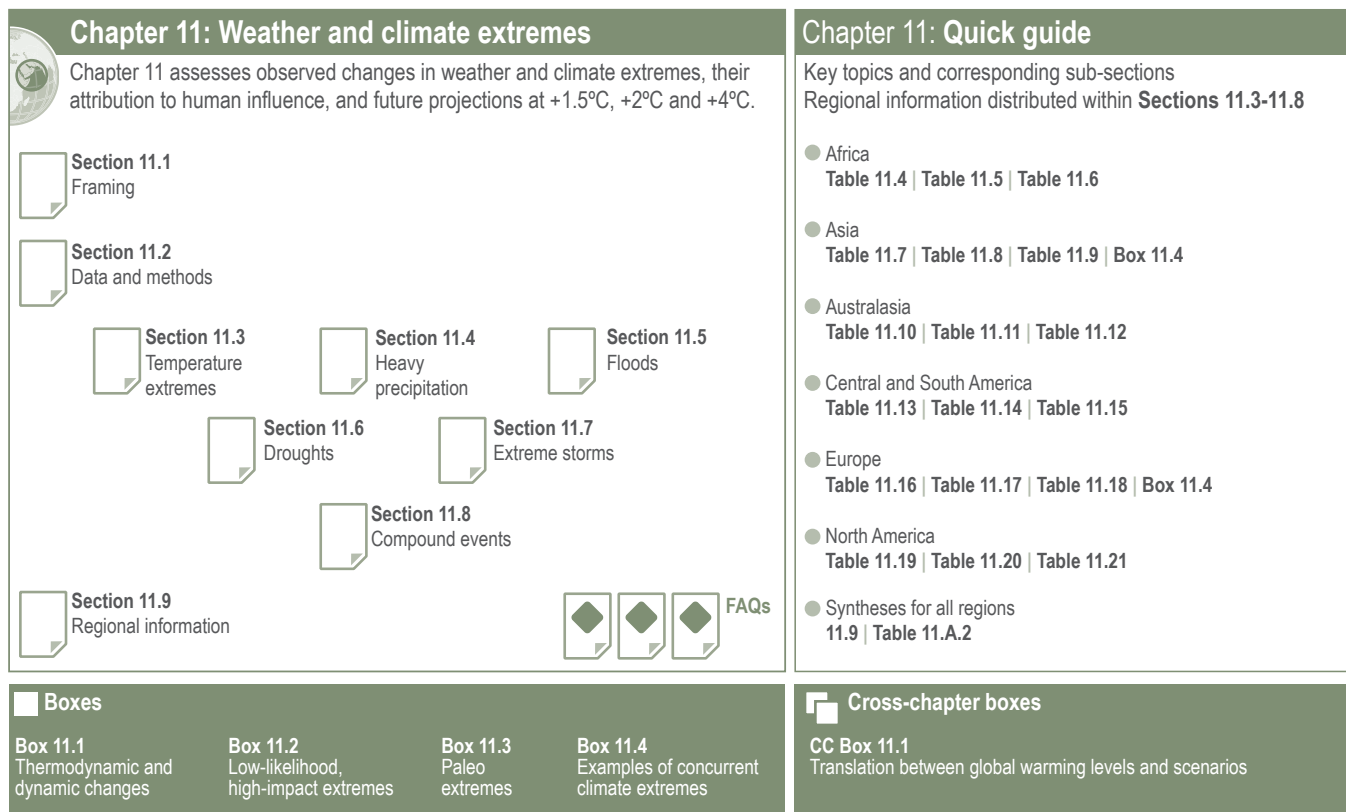
Figure 11.1 | Visual guide to Chapter 11.
