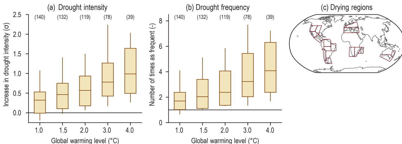
Figure 11.18 | Projected changes in (a) the intensity and (b) the frequency of drought under 1°C, 1.5°C, 2°C, 3°C, and 4°C global warming levels relative to the 1850–1900 baseline. (c) Summaries are computed for the AR6 regions in which there is at least medium confidence in an increase in agriculture/ecological drought at the 2°C global warming level ('drying regions'), including Western North America, Central North America, Northern South America, North-Eastern South America, South American Monsoon, South-Western South America, Southern South America, West and Central Europe, Mediterranean, West Southern Africa, East Southern Africa, Madagascar, Eastern Australia, Southern Australia. Caribbean is not included in the calculation because the number of land grid points was too small. A drought event is defined as a 10-year drought event whose annual mean soil moisture was below its 10th percentile from the 1850–1900 base period. For each box plot, the horizontal line and the box represent the median and central 66% uncertainty range, respectively, of the frequency or the intensity changes across the multi-model ensemble, and the 'whiskers' extend to the 90% uncertainty range. The line of zero in (a) indicates no change in intensity, while the line of one in (b) indicates no change in frequency. The results are based on the multi-model ensemble estimated from simulations of global climate models contributing to the Coupled Model Intercomparison Project Phase 6 (CMIP6) under different Shared Socio-economic Pathway (SSP) forcing scenarios. Intensity changes in (a) are expressed as standard deviations of the interannual variability in the period 1850–1900 of the corresponding model. For details on the methods see Supplementary Material 11.SM.2. Further details on data sources and processing are available in the chapter data table (Table 11.SM.9).
