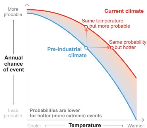
FAQ 11.3, Figure 1 | Changes in climate result in changes in the magnitude and probability of extremes. Example of how temperature extremes differ between a climate with pre-industrial greenhouse gases (shown in blue) and the current climate (shown in orange) for a representative region. The horizontal axis shows the range of extreme temperatures, while the vertical axis shows the annual chance of each temperature event’s occurrence. Moving towards the right indicates increasingly hotter extremes that are more rare (less probable). For hot extremes, an extreme event of a particular temperature in the pre-industrial climate would be more probable (vertical arrow) in the current climate. An event of a certain probability in the pre-industrial climate would be warmer (horizontal arrow) in the current climate. While the climate under greenhouse gases at the pre-industrial level experiences a range of hot extremes, such events are hotter and more frequent in the current climate.
