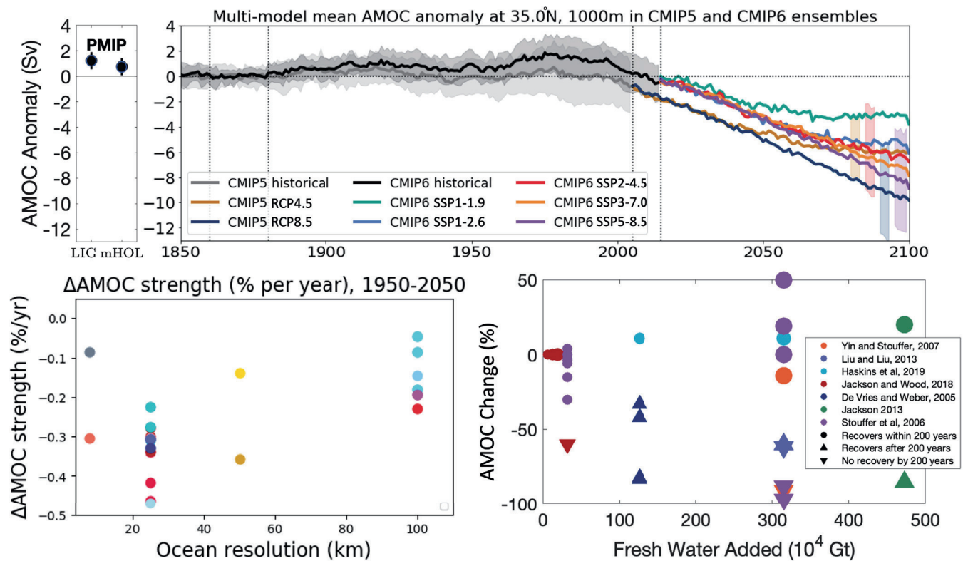
Figure 9.10 | Atlantic Meridional Overturning Circulation (AMOC) strength in simulations and sensitivity to resolution and forcing. (Top left) AMOC magnitude (units: Sverdrup (Sv) = 10 9 kg s -1 ) in Paleoclimate Modelling Intercomparison Project (PMIP) experiments. (Top right) Time series of AMOC from Coupled Model Intercomparison Project Phase 5 and 6 (CMIP5 and CMIP6) based on (Menary et al., 2020b). (Bottom left) Percent change in AMOC strength per year at different resolutions over the 1950–2050 period with colours for model families (Roberts et al., 2020). (Bottom right) A compilation of percentage changes in the simulated AMOC after applying an additional freshwater flux in the subpolar North Atlantic at the surface for a limited time (de Vries and Weber, 2005; Stouffer et al., 2006; Yin and Stouffer, 2007; Jackson, 2013; Liu and Liu, 2013; Jackson and Wood, 2018; Haskins et al., 2019). Symbols indicate whether the AMOC recovers within 200 years (circles), is starting to recover (upwards arrow), or does not recover within 200 years (downwards arrow). Symbol size indicates rate of freshwater input. Further details on data sources and processing are available in the chapter data table (Table 9.SM.9).
