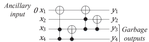
Fig. 1. Reversible circuit implementation of a full adder.
