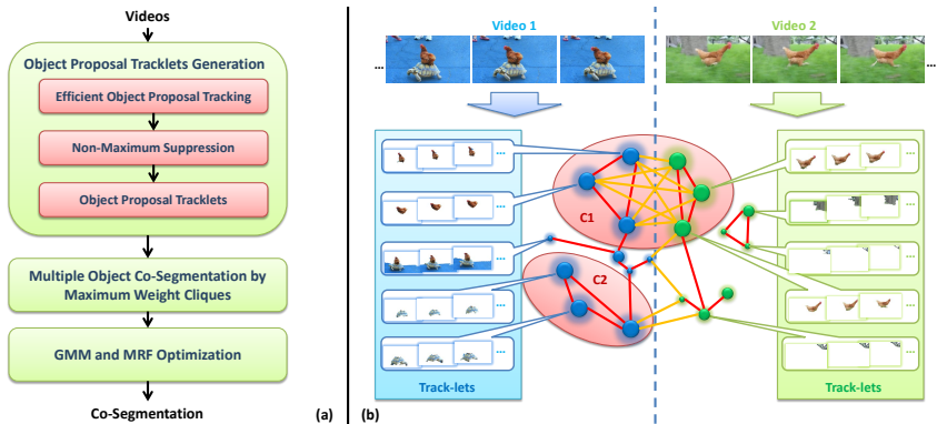
Fig. 1. (a) Shows the framework of the proposed method. (b) Shows the formulation of the Regulated Maximum Weight Cliques (RMWC) for object proposal tracklets. In this example, we generate ‘object proposal’ tracklets for two videos and use weighted nodes to represent them. Edges are built between similar nodes, and there are two types of edges (intra-video edges: red; inter-video edges: orange). In this example, the first two maximal cliques which have highest weights are obtained ( C1 and C2 ). C1 contains all the segments for ‘chicken’ from two videos and C2 contains all the segments for ‘turtle’ in video 1.
