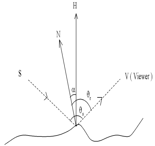
Fig. 3. Specular reflection geometry.
