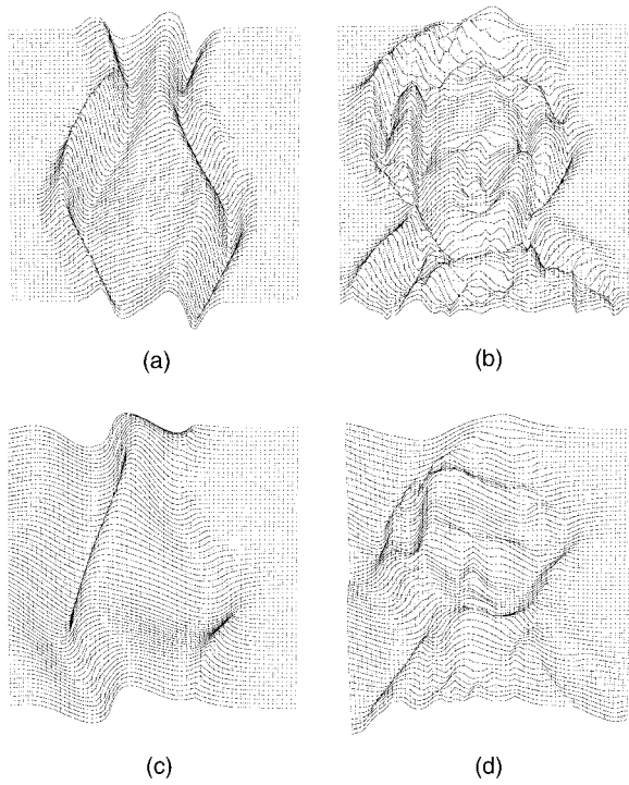
Fig. 7. Results for Zheng and Chellappa's method on synthetic images: (a) vase, (b) Mozart, (a1) and (b1) show the results for test images with light source (0, 0, 1) . (a2) and (b2) show the results for test images with light source (1, 0, 1) .
