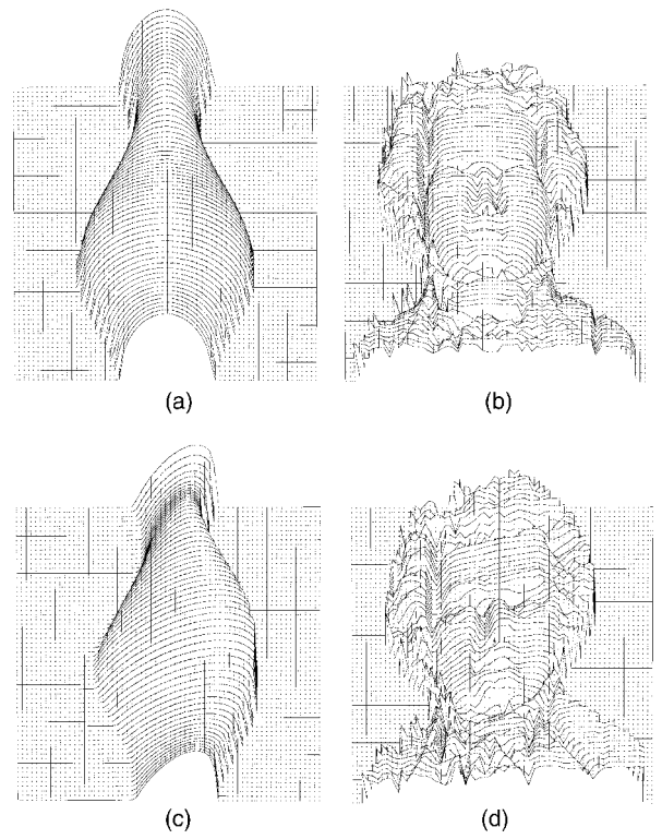
Fig. 12. Results for Tsai and Shah's method on synthetic images: (a) vase, (b) Mozart. (a1) and (b1) show the results for test images with light source (0, 0, 1). (a2) and (b2) show the results for test images with light source (1, 0, 1).
