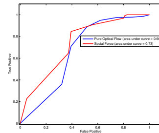
Figure 11. The ROCs of abnormal behavior detection in the web dataset.
