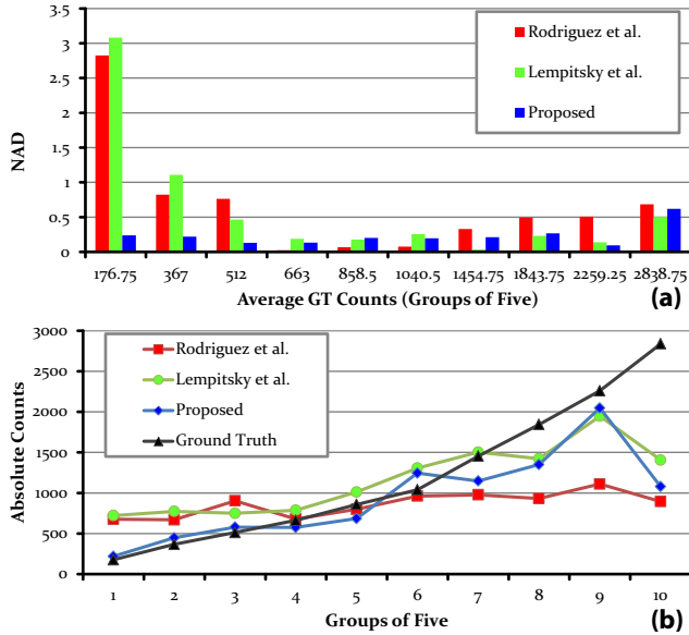
Figure 9: Analysis of comparison: Bars and lines in red depict [20], green show [13], blue shows the results using proposed approach, while ground truth is shown in black. (a) shows Normalized Absolute Difference (an error measure) and (b) shows the actual and estimated counts.
