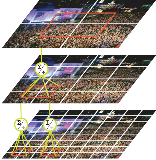
Figure 5: The figure shown multi-scale Markov random Field for inferring counts for the entire image. The patches in each layer have independent data terms, thus requiring a simultaneous solution for all layers.
