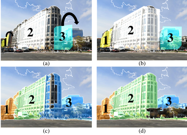
Figure 7: (a) shows the initial projections obtained using the original meta-data provided in the EXIF-tag of the image. (b) shows the projections after the iterative refinement. As illustrated, projection 1 is an example of a misaligned projection and therefore its corresponding segmentation result shown in (c) is inaccurate. On the other hand, 2 is a relatively reliable projection-segmentation pair. (d) shows segmentation results obtained using the updated projections in (b). Comparing the segmentation results for segment 3 before and after alignment, it is easy to see the effect of our updating step. Projection-segment pair 1 and mostly 2 are being used as an anchor point for aligning 3 which is the least accurate.
