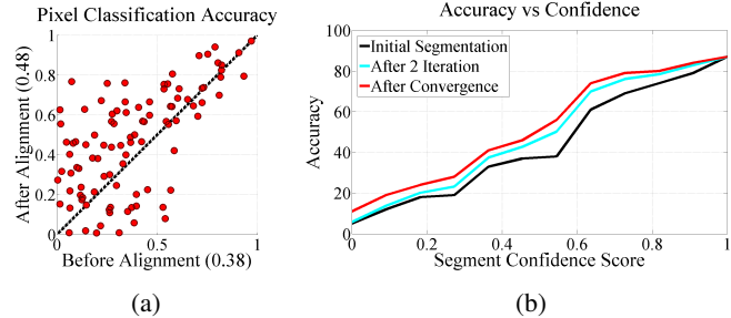
Figure 9: The scatter plot in (a) shows the accuracy improvement due to our updated projections. Each point represents the overall segmentation accuracy in one of the images before and after our iterative method. (b) shows the amount of improvement gained in each iteration vs the reliability of the semantic objects.
