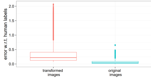
Figure 6: Deviations from the human labels for images that violate the metamorphic relation (see Equation 2) is higher compared to the deviations for original images. Thus, these synthetic images have a high chance to show erroneous behaviors.
