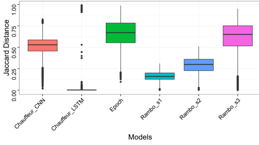
4.1 Difference in neuron coverage caused by different image transformations
