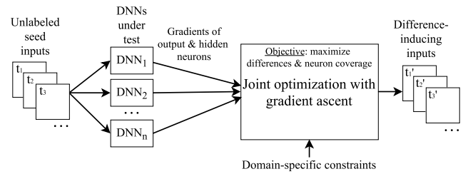
Figure 5: DeepXplore workflow.
