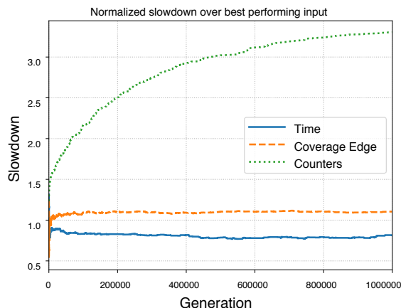
Figure 10: Comparison of the slowdown achieved by SlowFuzz under different guidance mechanisms, when applied on the OpenBSD quicksort implementation of Section 5.2, for an input size of 64 bytes, after 1 million generations (average of 100 runs).
