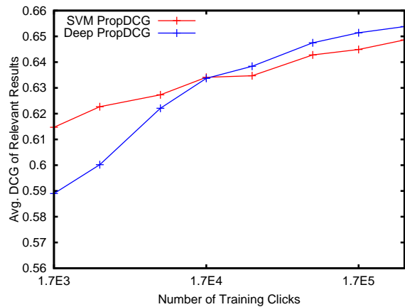
Figure 8: Test set Avg DCG performance for SVM PropDCG and Deep PropDCG ( \eta = 1 , \epsilon_- = 0.1 )
