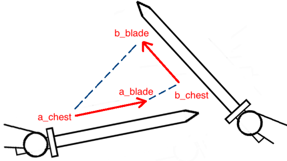
Figure 1: A metaphorical illustration of the blade-chest model for intransitivity. Player a and player b are in a sword duel. Player a 's blade is closer to player b 's chest than vice versa, as shown by the two blue dashed lines. This illustrates how player a has a better chance of winning than player b .
