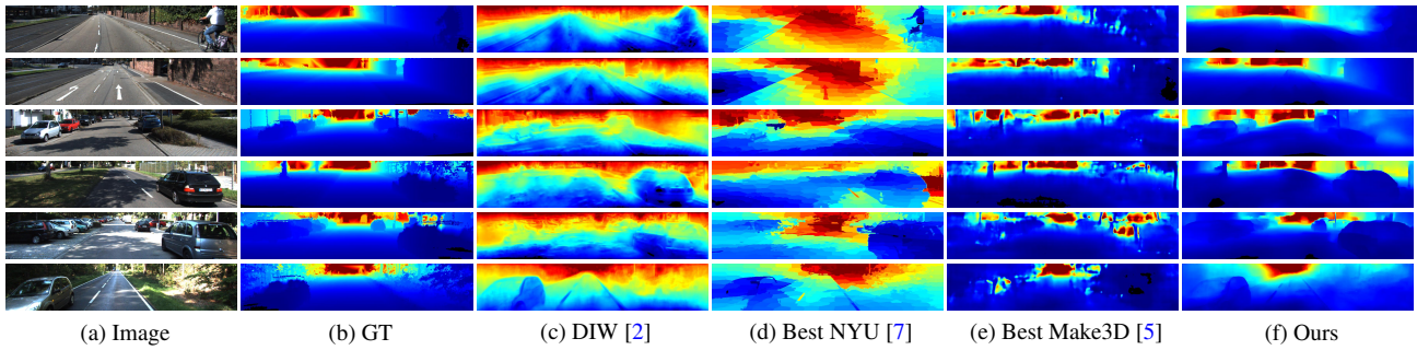
Figure 8: Depth predictions on KITTI. (Blue=near, red=far.) (a) Input photo. (b) Ground truth (c) DIW-trained network predictions [2]. (d) Best NYU-trained network predictions [7] (e) Best Make3D-trained network predictions [5]. (f) Our MD-trained network predictions. None of the models were trained on KITTI data.
