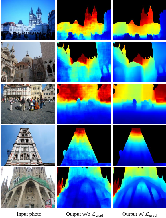
Figure 3: Depth predictions with and without \mathcal{L}_{grad} . \mathcal{L}_{grad} encourages the prediction to match the depth gradient of the ground truth.
