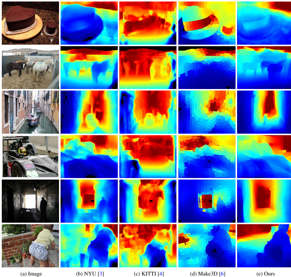
Figure 9: Depth predictions on the DIW test set. (Blue=near, red=far.) (a) Input photo. (b) Best NYU-trained network predictions [3]. (c) Best KITTI-trained network predictions [4] (d) Best Make3D-trained network predictions [6]. (e) Our MD-trained network predictions. None of the models were trained on DIW data.
