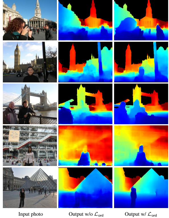
Figure 4: Depth predictions with and without \mathcal{L}_{ord} . \mathcal{L}_{ord} corrects ordinal depth relations for hard-to-construct objects such as people.
