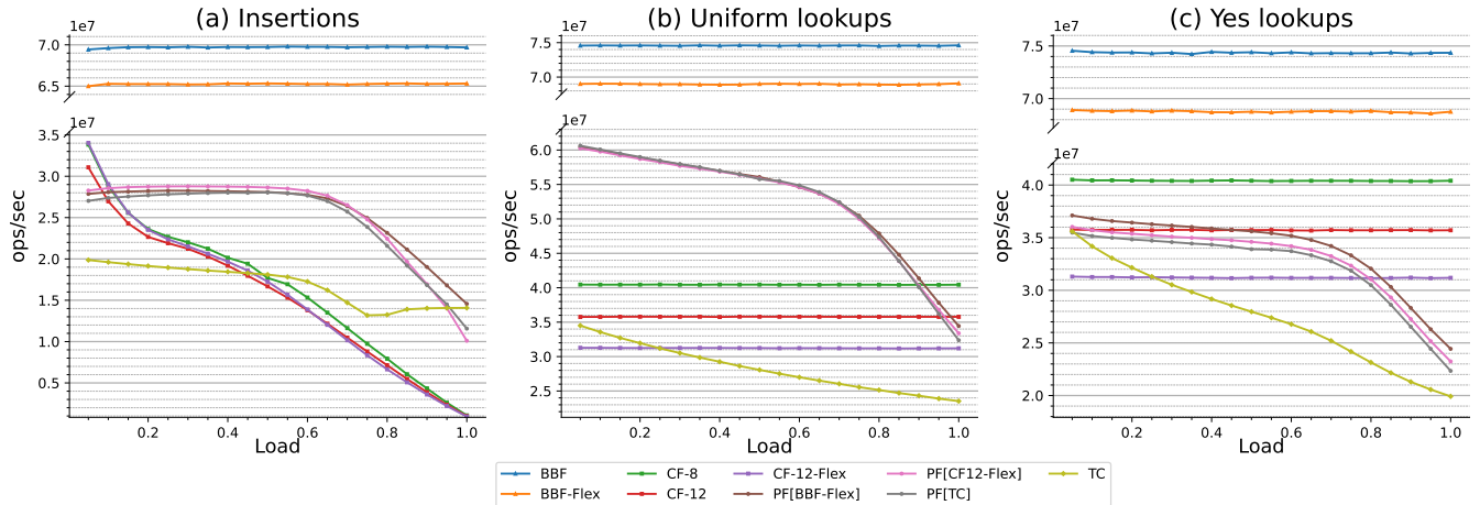
Figure 2: Throughput comparison as filter load increases ( X -axis shows the fraction of n = 2^{28} \cdot 0.94 elements inserted so far).
