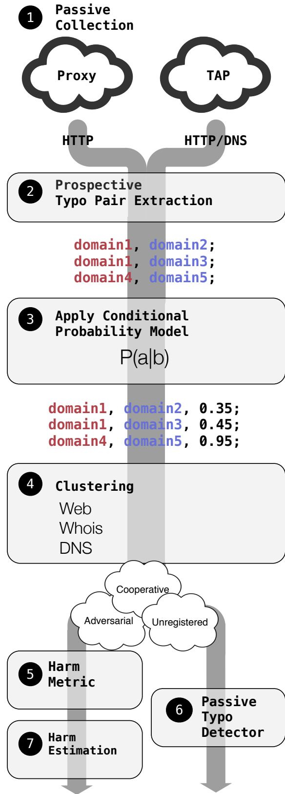
Fig. 1. Methodology overview.
