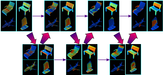
Figure 3: Information flow in weakly-supervised WU-Net, captured as layer activation maps (red: high) for detecting chair arms/backs, ship sails, and plane engines. Shallow U’s prevent over-summarization, and the signal is not lost by repeated concatenations from distant layers, unlike a deep U (Figure 4).
