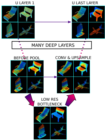
Figure 4: Arm, back, sail and engine signals are lost via over-summarization and ambiguous high-resolution concatenations in a weakly-supervised deep U-Net.
