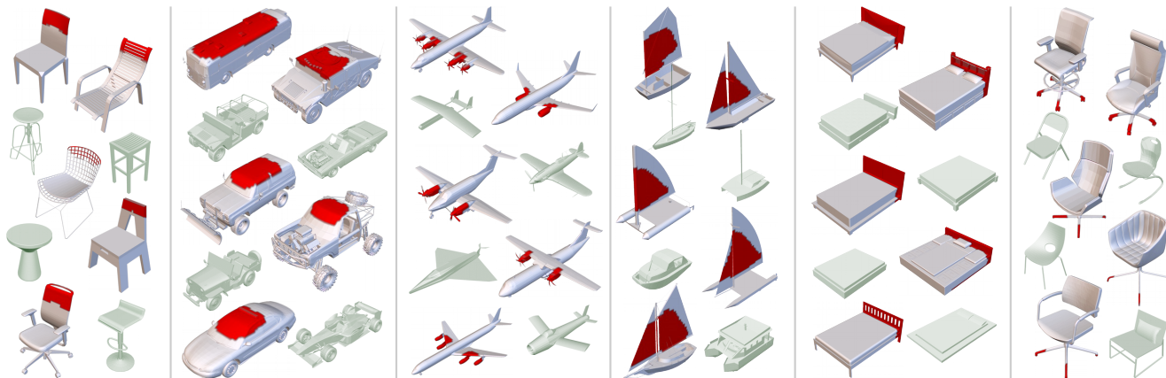
Figure 7: Examples of weakly supervised segmentation by WU-Net. Left to right: detecting chair backs, car roofs, wing-mounted airplane engines/propellers, ship sails, bed heads, and chair swivels.
