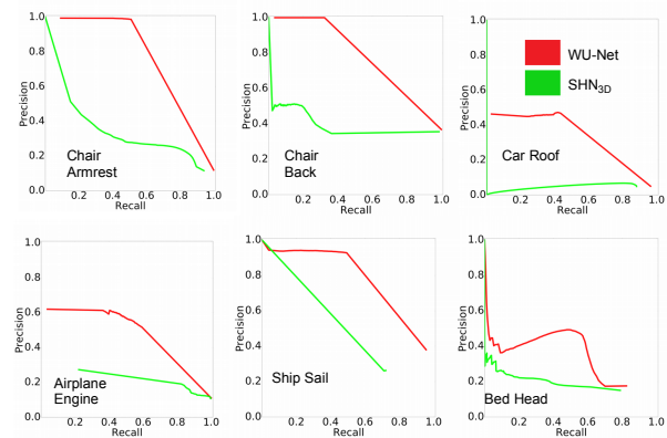
Figure 11: WU-Net (red) consistently outperforms a Stacked Hourglass Network SHN 3D (3 deep U's without low resolution skip connections between different U's, green) on all categories (on training shapes, outputs symmetrized).
