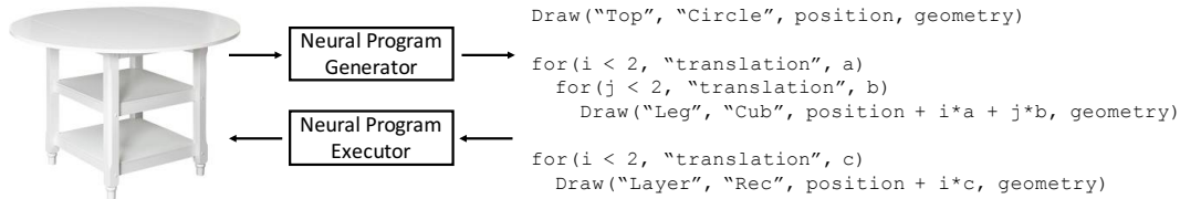
Figure 24: The shape program representation aims to explain an input shape with high-level programs that encodes basic parts, as well as their structure such as repetition [TLS* 19].
