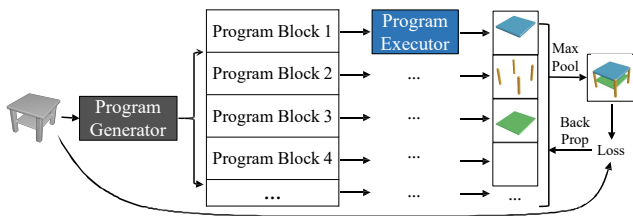
Figure 25: The model for inferring and executing 3D shape programs [TLS* 19]. At each step, it infers the next program block (e.g. a set of cuboids as legs), executes the program block, and compares the current shape with the input to suggest what to synthesize next.
