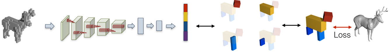
Figure 23: Overall pipeline of reconstructing 3D shapes via a set of geometric primitives [TSG* 17]. The model learns to decompose shapes into primitives and uses Chamfer distance, which computes the difference between the reconstructed shape with the input shape, as the loss function to train the inference network.
