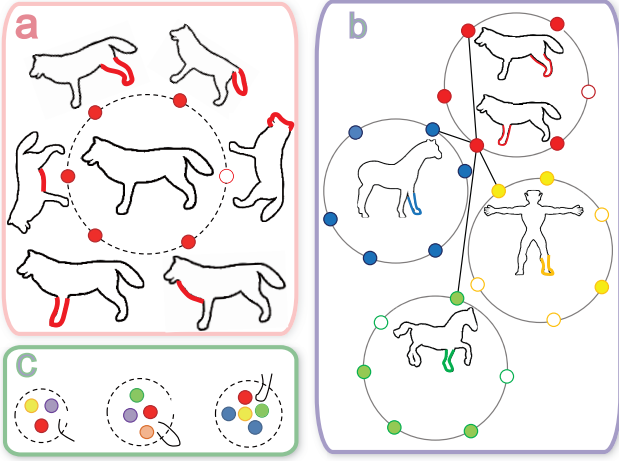
Figure 4: Illustration of our randomized compound kNN graph. In this figure, a solid circle represents a valid section and a dashed circle represents an invalid one. Given a contour (taken as a node of our randomized compound kNN graph), we first generate several sections (a). Then, we find the nearest neighbors for each section and establish edges between the parent contours of these sections (b). Finally, we find valid sections and cluster them (c).
