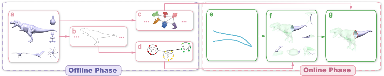
Figure 2: Pipeline of our system. In the offline phase, for each model in a given shape database (a), we first extract its boundary contours (b). We then construct the super-face graph for each model (c), and organize the boundary contours of all models into a randomized compound k -NN graph (d). In the online phase, the user draws a rough sketch to convey his/her design intent (e). Regions of database shapes matching the sketch are rapidly identified via partial shape matching (f). A selected part is further refined to optimize its boundary and better match the sketch (g)
