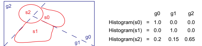
Figure 7: Distributions of super-faces on segments. s_0, s_1, and s_2 are the super-faces. g_0, g_1, and g_2 are the segments generated by the randomized segmentation on the shape.
