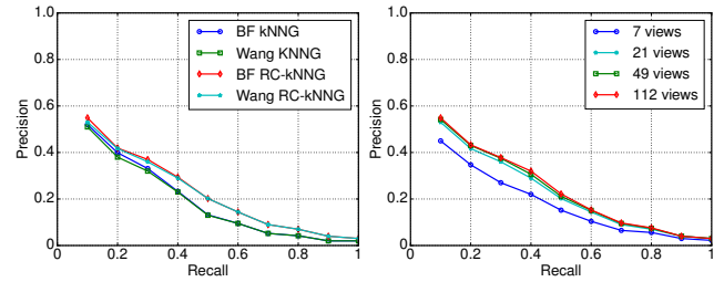
(a) Different retrieval methods (b) Different camera view settings
