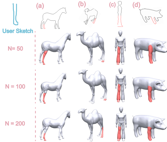
Figure 19: Improvement in part quality with increasing super-face count ( N ). With more super-faces, the extracted part fits the user's sketch better and better.
