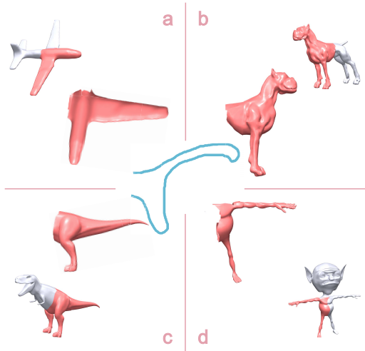
Figure 1: Given a roughly drawn sketch, our algorithm rapidly searches a shape database to identify and extract customized parts that match the sketch. No presegmentation is required: the retrieved parts can be irregular and not match any standard segmentation.
