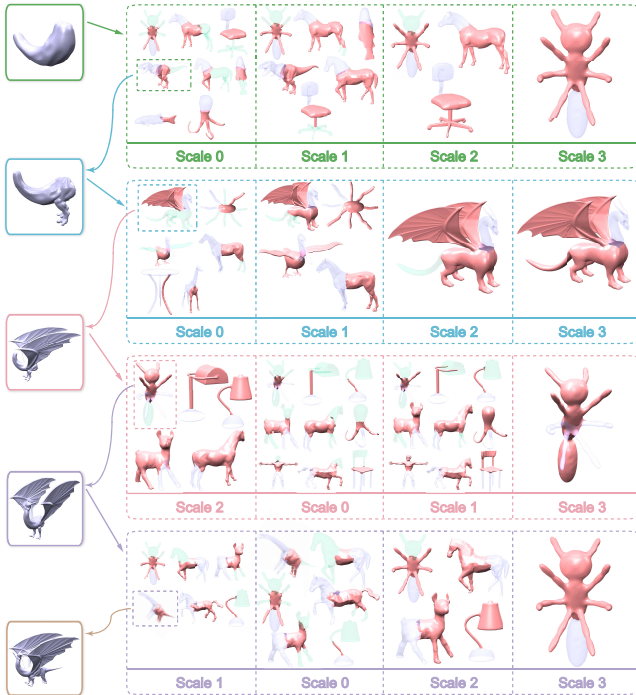
Figure 15: An example of multi-scale part suggestion. The initial shape and subsequent working models, used as queries, are listed in the left column. On the right, we show the suggested parts (red) at different scales for each modeling step. The parts corresponding to the queries are marked in light blue. The other parts are marked in light green.
