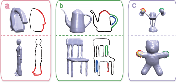
Figure 8: Illustrations of the complexity of contours and their relationship. Depth-discontinuous contour sections are shown in (a). Topologically different contour sections are illustrated in (b). Isolated contour sections are shown in (c).
