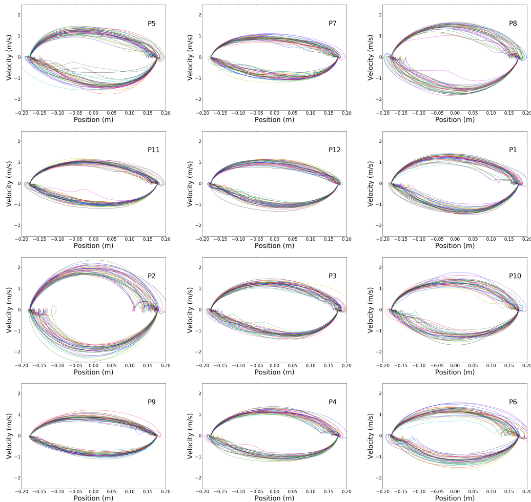
Fig. 5. Phase space plots of all 12 participants for pointing on 1.38 mm targets at 353 mm distance (ID 8). The plots are sorted by deceleration slope from left to right. Movements on the left are more ballistic, with a relatively symmetric acceleration and deceleration slope. Movements on the right have a less steep deceleration, indicating that the participants are correcting their movement while they are decelerating (c.f. Figure 6). There is considerably more undershooting than overshooting. Finally, the spring-mass properties of the human hand sometimes lead to small ‘loopings’ when the mouse stops (e.g., P5). For clarity, failed trials are not shown.
