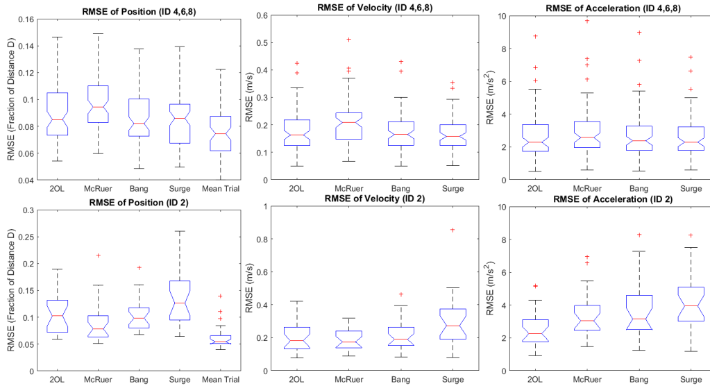
Fig. 9. RMSE of position (left column), velocity (middle column) and acceleration (right column) of different models. ID 4,6,8 are shown together in the top row and ID 2 is shown separately in the bottom row. For position, RMSE is shown as a fraction of distance between targets, for velocity in \text{ms}^{-1} and for acceleration in \text{ms}^{-2} . Differences among models are small, but Bang-bang shows best fit and McRuer the worst. Note the difference in scale between the top and bottom rows. For position, ID 2, one outlier of Surge is not shown.
