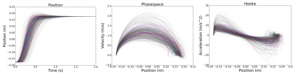
Fig. 4. An overview of dynamics in the task of pointing at 1.38 mm targets at 353 mm distance (ID 8). Left: Time series; Middle: Phase space plots; Right: Hooke plots. For clarity, failed trials are not shown.
