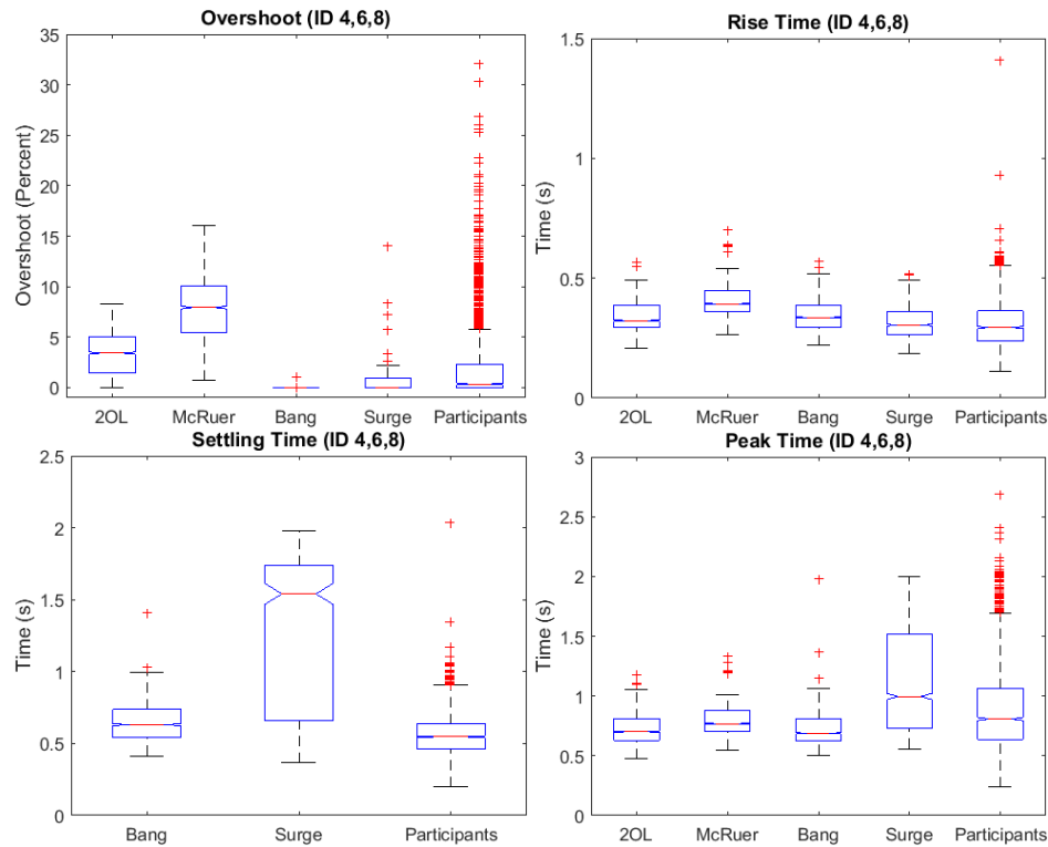
Fig. 17. Step response parameters of the four models and the participants. The plot exposes distinct patterns among the models. From top left to bottom right: Overshoot, Rise Time, Settling Time, Peak Time, respectively. Overshoot has 6 hidden outliers.
