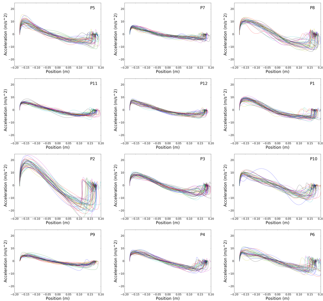
Fig. 6. Hooke plots of all 12 participants for pointing on 1.38 mm targets at 353 mm distance (ID 8). The order of participants is the same as in Figure 5. For participants on the left, the Hooke plot has a more symmetric N shape, while for those on the right, the deceleration is less steep than the acceleration. Plots on the left show higher accelerations than plots on the right.
