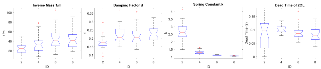
Fig. 18. Parameters of 2OL by ID. From left to right: \frac{1}{m} , d , k , dead time. “Mass” m decreases, the damping factor d increases and the spring constant k decreases with increasing ID. This explains the slower reaction but reduced overshooting and less oscillations as the ID increases, leading in total to faster settling on small targets.
