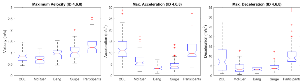
Fig. 13. Left: Maximum velocity of different models and participants (ID 4,6,8). Middle: Maximum acceleration of different models and participants (ID 4,6,8). Right: Maximum deceleration of different models and participants (ID 4,6,8).
